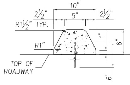
EXTRUDED CURB
