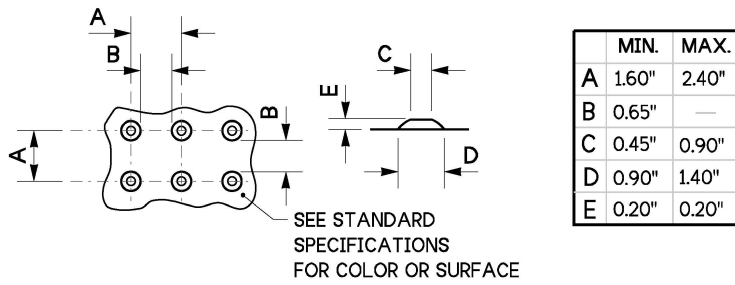
TRUNCATED DOME DETAILS SEE NOTE 3
