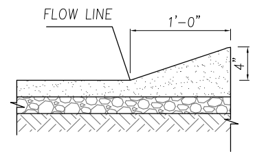
HMA WEDGE CURB
