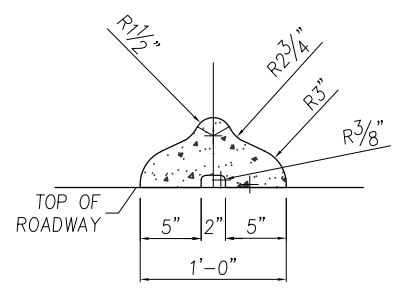
TYPE "C" CURB
