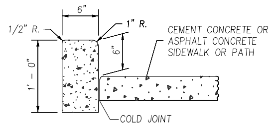
PEDESTRIAN CURB
