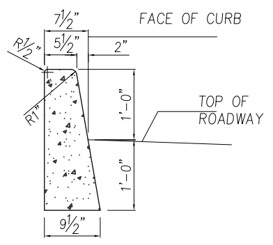
TRUCK BARRIER CURB
