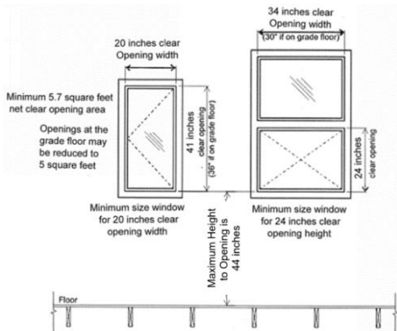
Minimum Emergency Egress and Rescue Opening Dimensions
